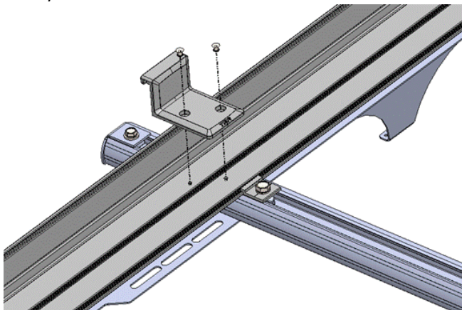
Figure 4 Ladder Slide Buffer (5)
