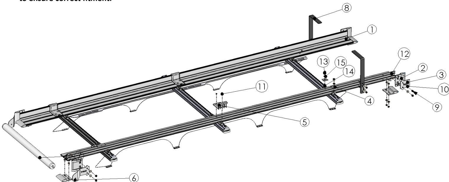
Figure 1 Ladder Slide
