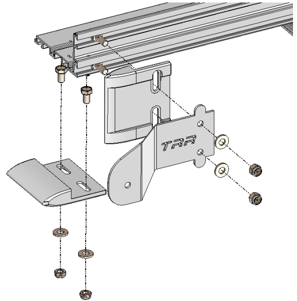
Figure 5 Tech Roller and Ladder Slide End
