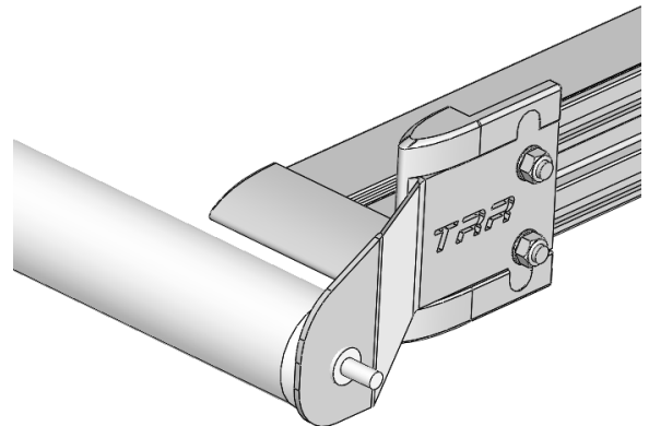
Figure 6 Stainless Roller
