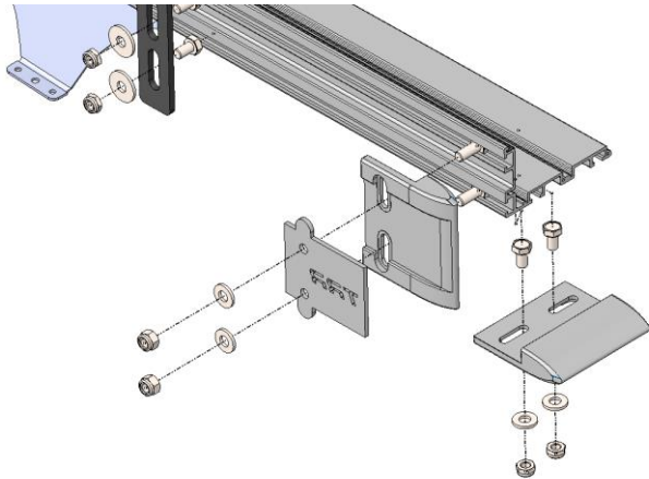
Figure 3 Ladder Slide End Caps (2)
