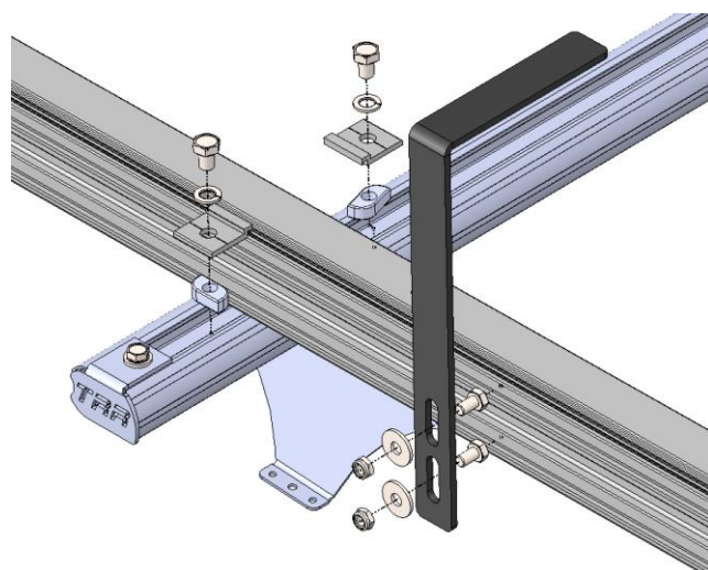
Figure 2 Ladder Slide Crossbar Anchor (4) and Ladder L Bracket (8)
